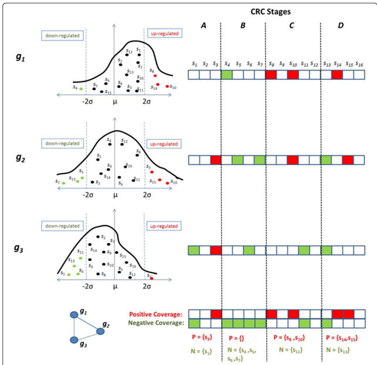
Figure 2 Illustration of the set-cover based algorithm for the identification of one-vs-all discriminative subnetworks. Here, the coverage provided by a hypothetical three-gene subnetwork is shown. In the left panel, the distribution of the expression levels of each gene across all samples is shown. We first compute the mean ( \mu ) and the standard deviation ( \sigma ) of this distribution for each gene g_i . Subsequently, we identify samples that are positively or negatively covered by each gene. A gene g_i with expression greater than \mu_i + \alpha * \sigma_i in a sample is said to positively cover that sample, while a gene g_i with expression less than \mu_i - \alpha * \sigma_i in a sample is said to negatively cover that sample (we set \alpha = 2 in our experiments). The negative and positive cover sets for each gene and the subnetwork composed of g_1 , g_2 and g_3 are shown on the right. In this example, this subnetwork negatively covers (all samples in) Stage B.
